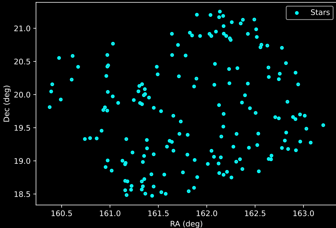
APOGEE DR17 Field: [K2_C4_173-23_btx] Proper Motion Vectors for Gaia Star Field (n= 173)
