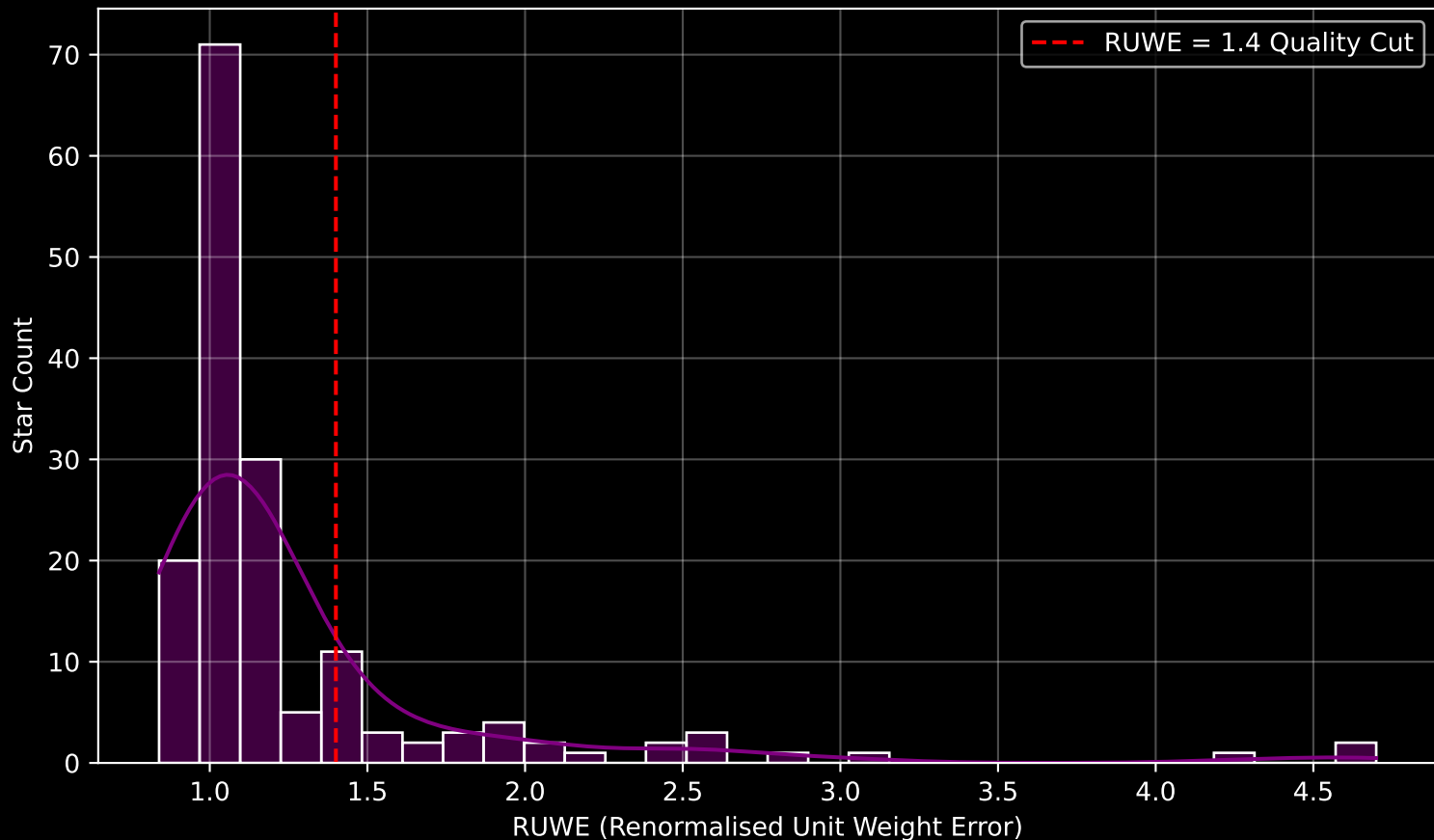
GAPOGEE DR17 Field [K2_C4_173-23_btx] RUWE Distribution (n= 162)
