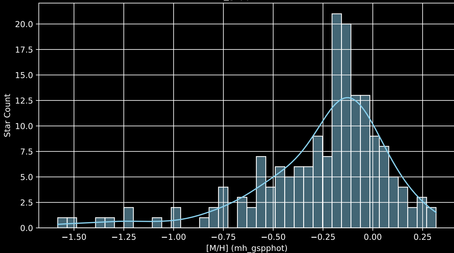
APOGEE DR17 Field: [K2_C4_173-23_btx [M/H] (mh_gspphot) (n= 171)
