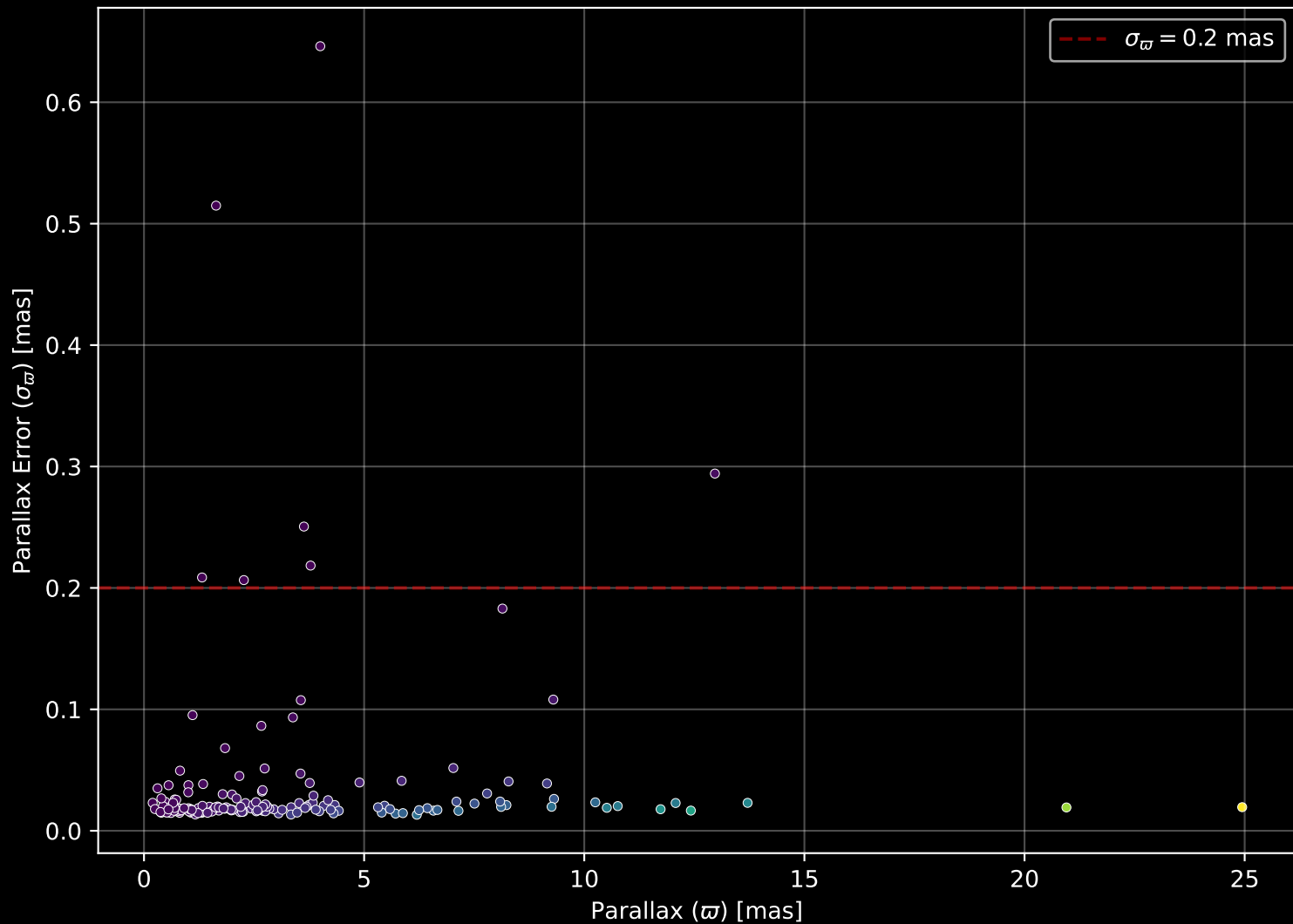
APOGEE DR17 Field: [K2_C4_173-23_btx] Parallax Quality (n= 173)
