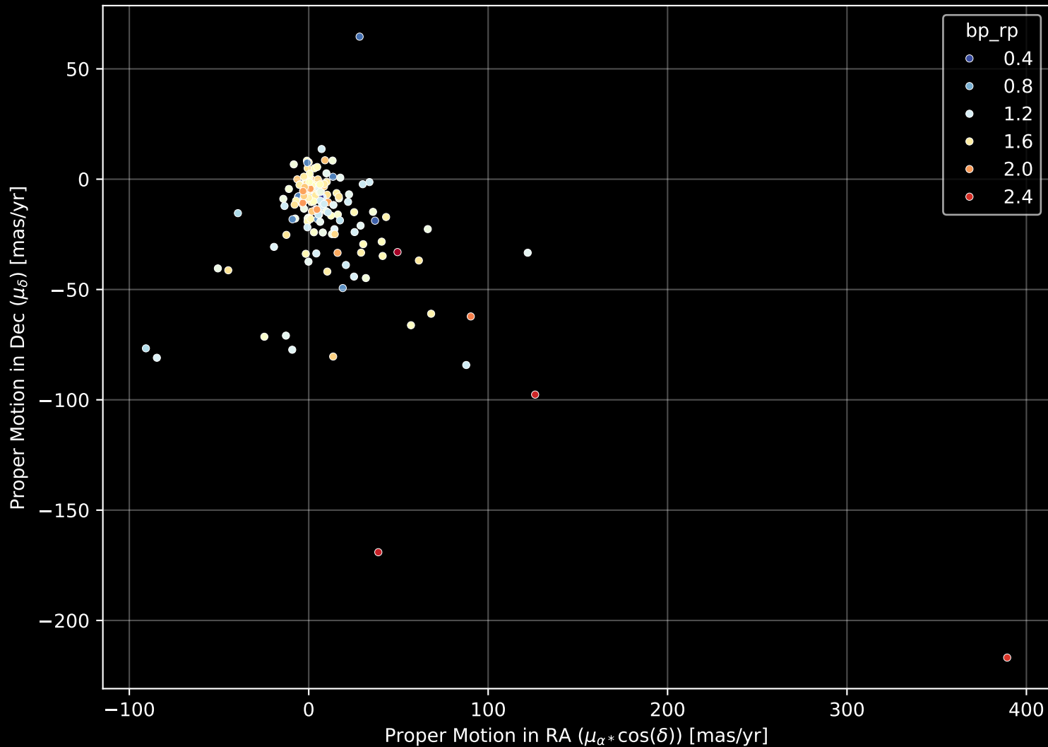
APOGEE DR17 Field: [K2_C4_173-23_btx] Proper Motion Diagram (n= 173)
