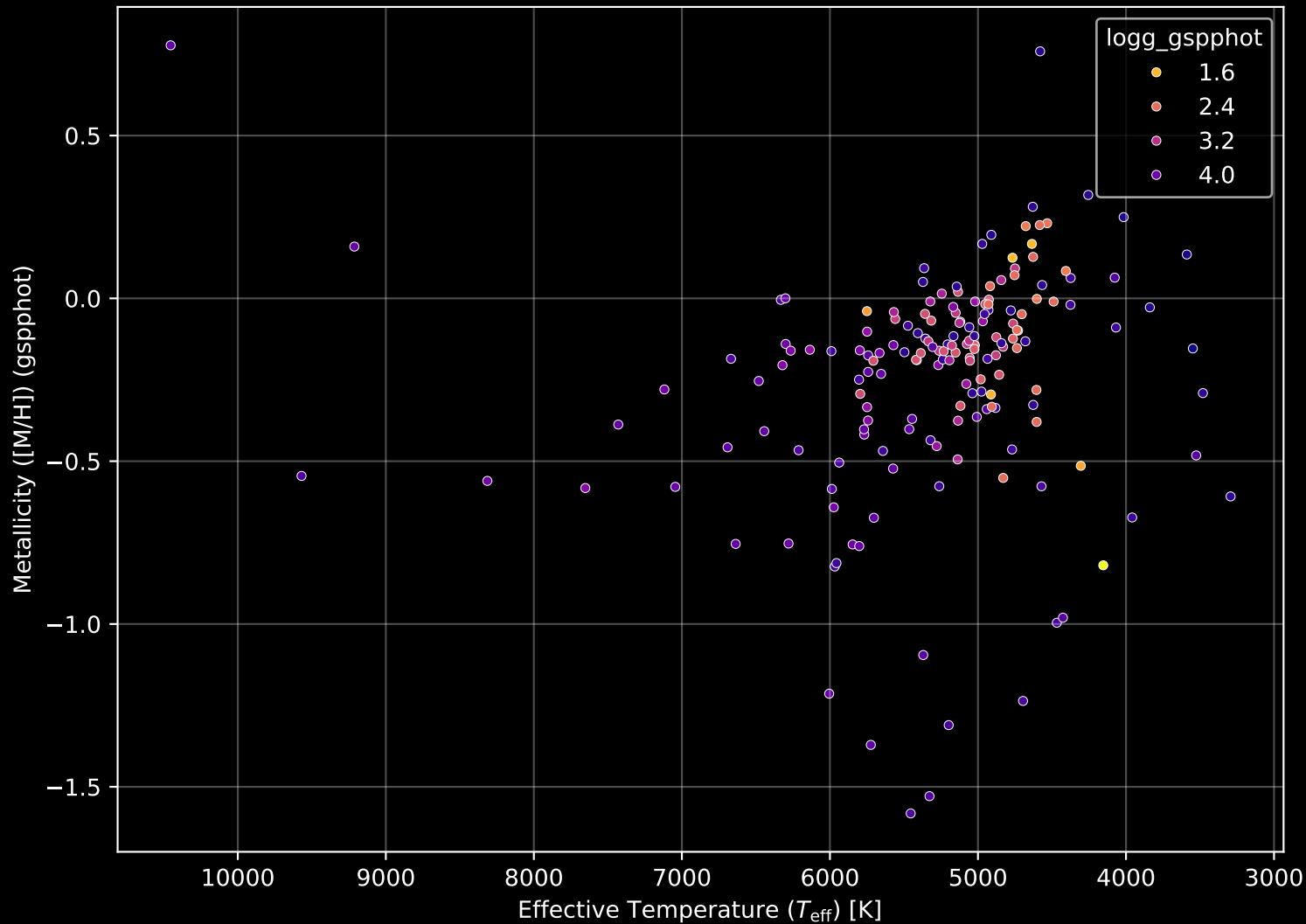
APOGEE DR17 Field: [K2_C4_173-23_btx] Stellar Population Parameters (n= 173)
