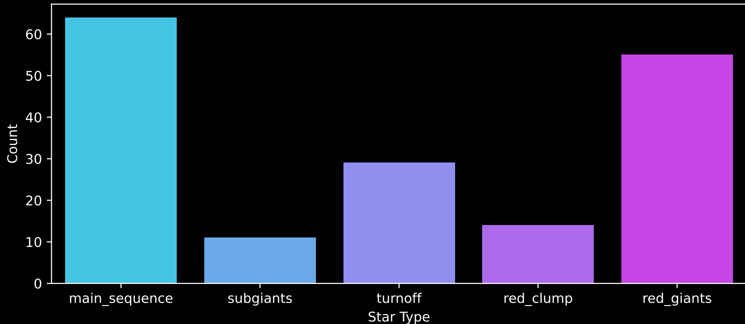
APOGEE DR17 Field: [K2_C4_173-23_btx] Count plot of Star Type
