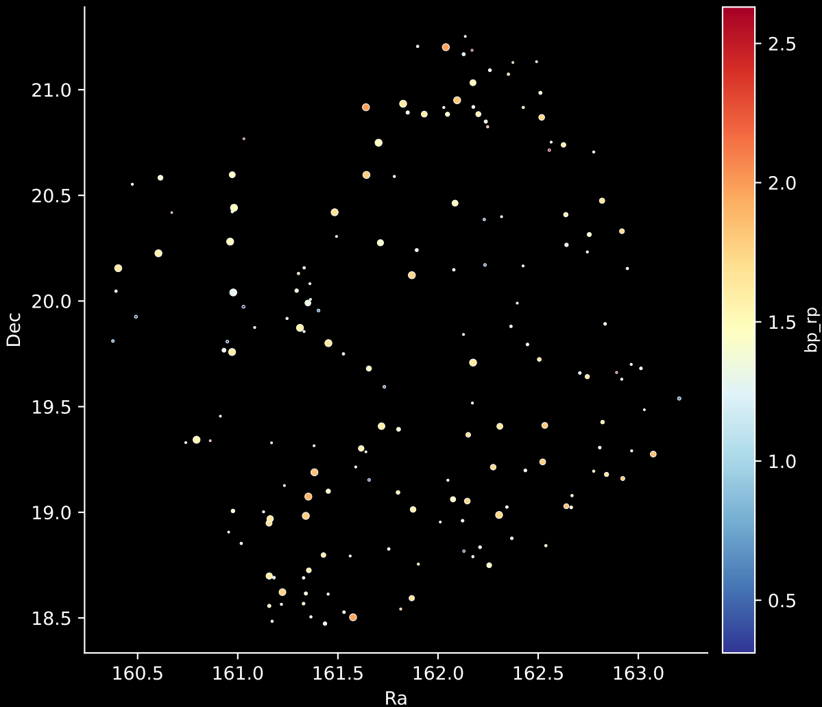
APOGEE DR17 Field: [K2_C4_173-23_btx] Stars: 173
